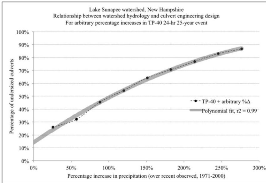
Figure 3-9. The hydrologic/hydraulic relationship between percentage change in precipitation and percentage change in undersized culverts.
