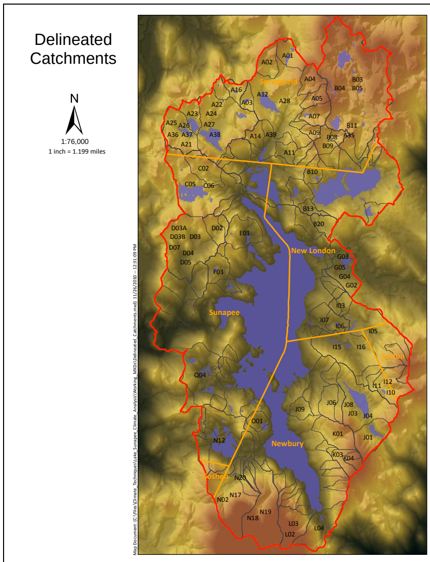
Figure 3-2. Modeled subcatchments identified and delineated. Note location of subcatchment/culvert A04, at the top center of the study site.
