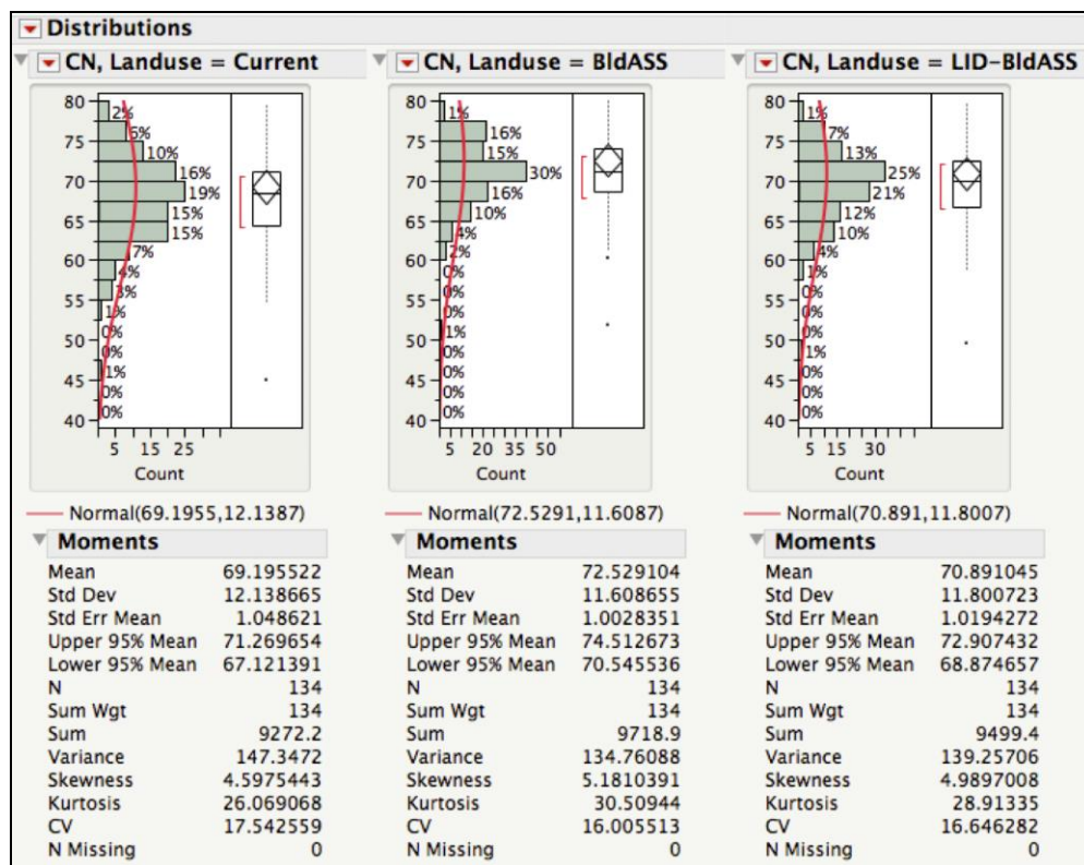
Figure 3-14b. Impact of landuse on curve number. BldASS is an abbreviation of the scenario buildout with all steep slopes included.
